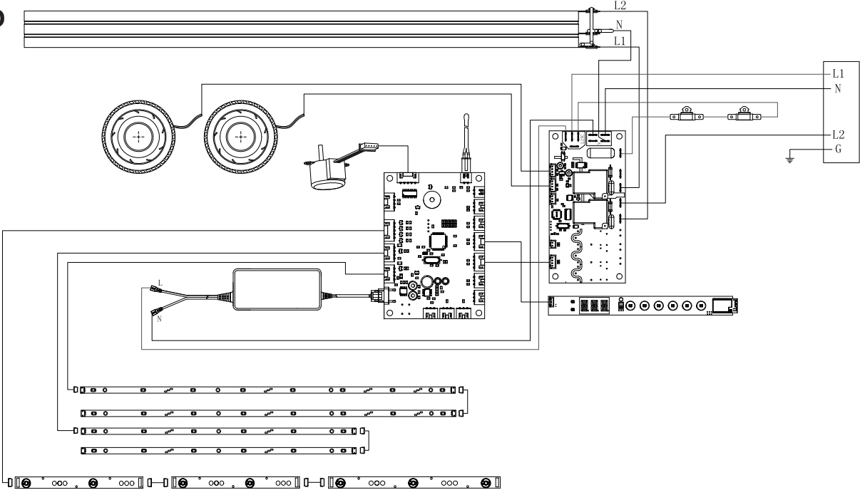
XLF5017-XD
